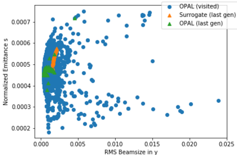
Beamsizes in y vs Normalized Emittance s.png
